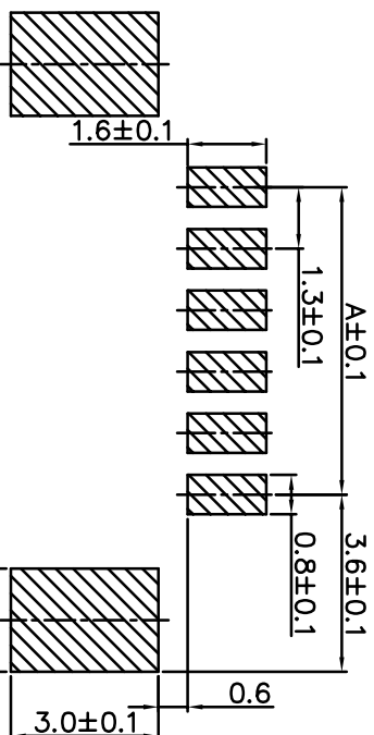
PCB LAYOUT
